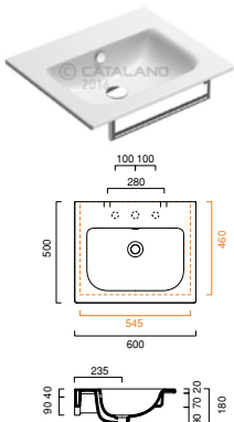
Sfera 60 CA160SFN00
