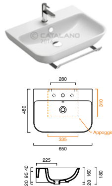
Sfera 65 CA165BSF00
