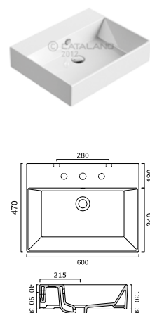
Premium 60 CA160VP00
