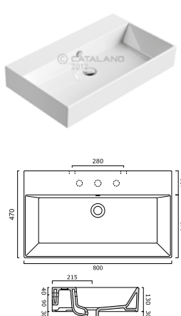
Premium 80 CA180VP00
