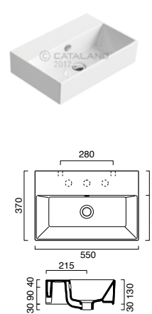
Premium 55 CA155VP00
