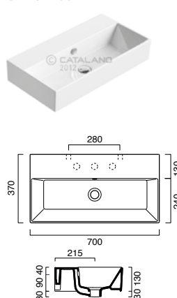
Premium 70 CA170VP00
