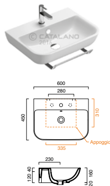
Sfera 60 CA160BSF00
