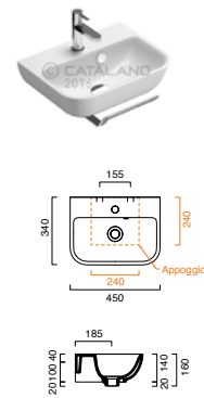
Sfera 45 CA145BSF00
