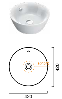
Velis 42 CA142APVL00
