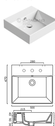
Premium 50 CA150VP00
