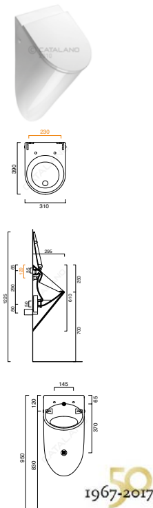
Urinal 39 CA1BIGBOY00
