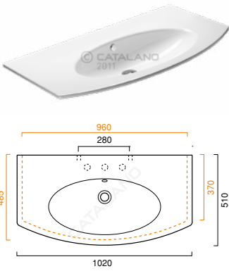
Velis 102 CA1102VL00
