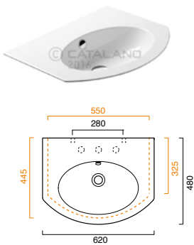
Velis 62 CA162VL00
