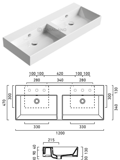
Premium 120 CA112VPD00
