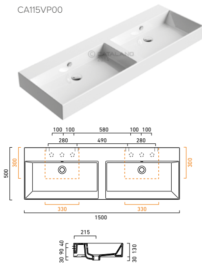
Premium 150 CA115VP00
